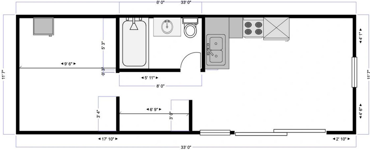
THE CLASSIC 1233SEB 380 Sq Ft | 12 x 33 | 1 Bed | 1 Bath
